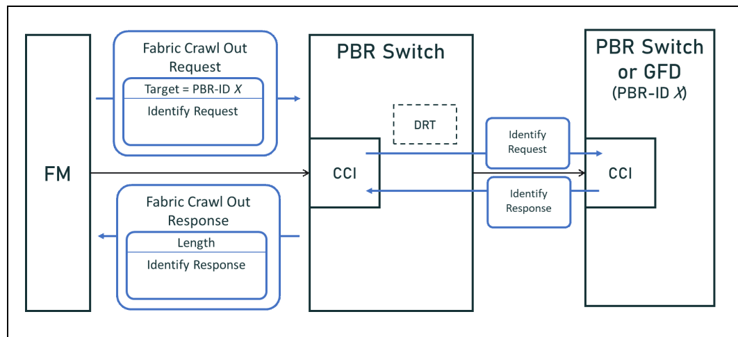
Figure 7-54. Tunneling Commands to Remote Devices
