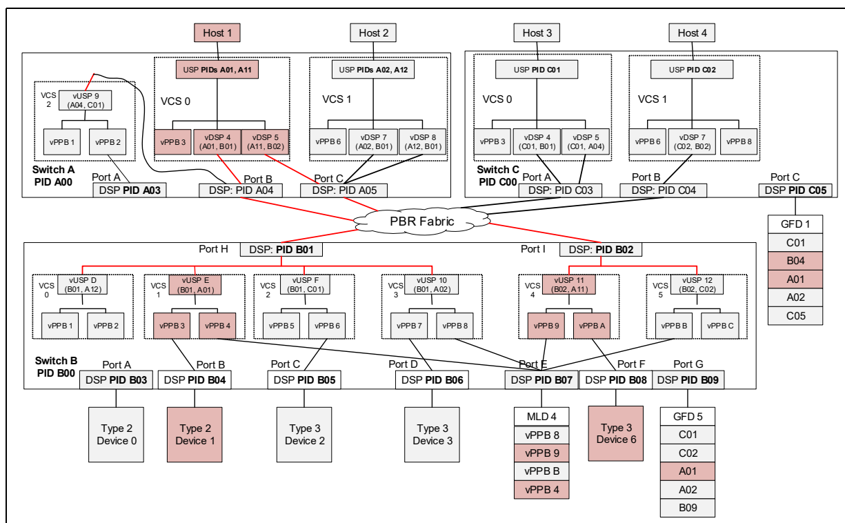
Figure 7-52. Single VH
